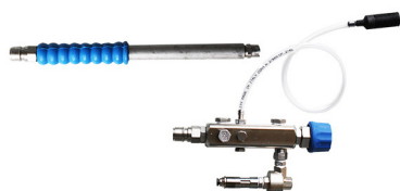
Compressed air foaming injector Cod. 10.3564.00
